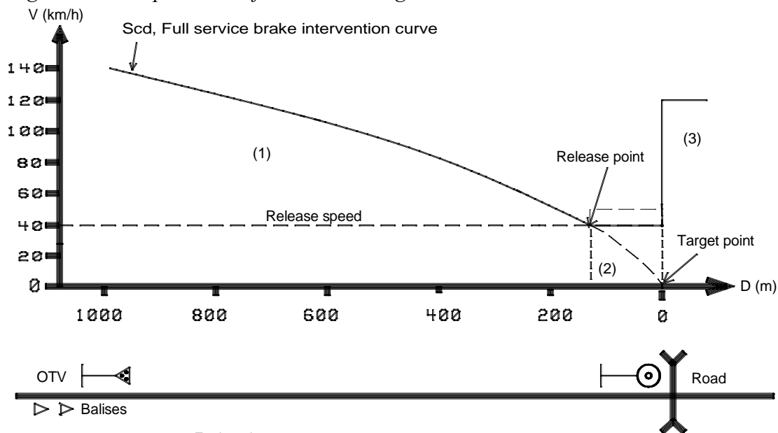
Figure 4.6-3. Supervision of a level crossing
