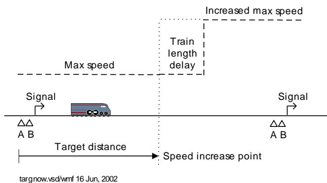
Figure 3.6-4. Preset speed increase
