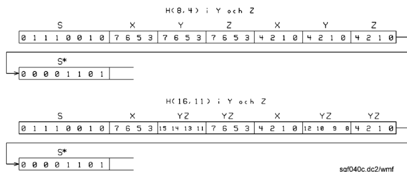
Figure 3.2-1. Telegram layout
