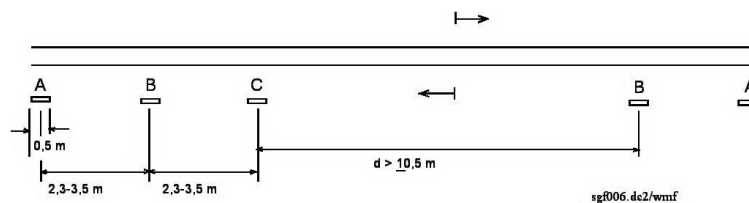
Figure 3.2-1. Distances between balises and balise groups
