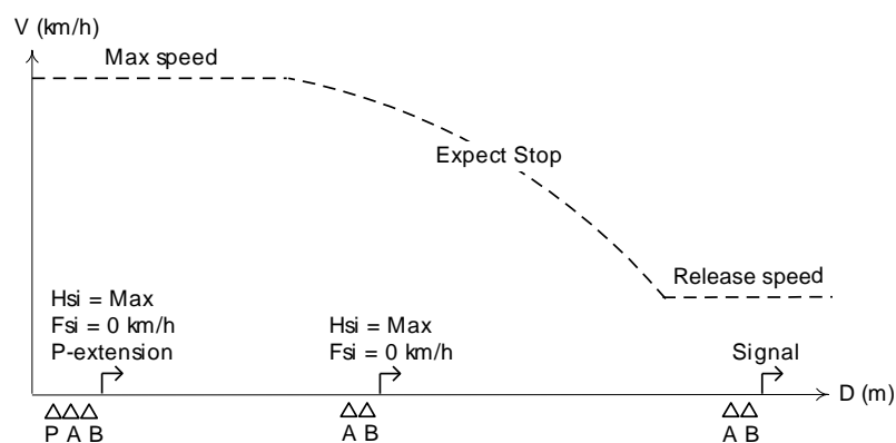
Figure 3.6-1. Example of a P-extension
